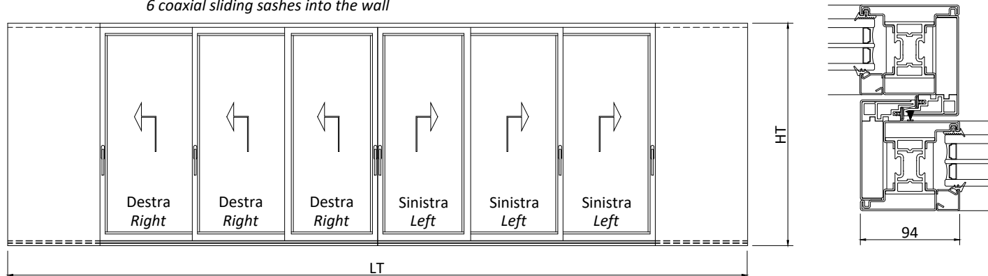
Schema | Type T3 6 ante scorrevoli coassiali a scomparsa 6 coaxial sliding sashes into the wall
