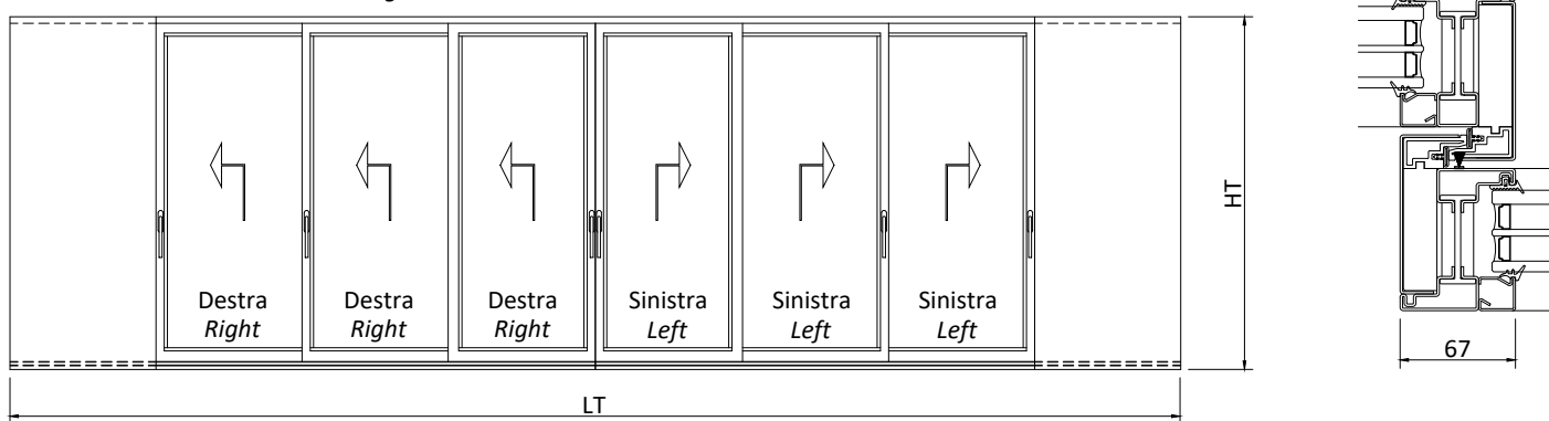
Schema | Type T3 6 ante scorrevoli coassiali a scomparsa 6 coaxial sliding sashes into the wall
