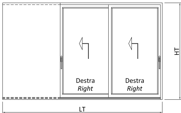
Schema | Type S2 2 ante scorrevoli a scomparsa 2 sliding sashes into the wall
