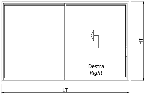
Schema | Type B 2 ante scorrevoli 2 sliding sashes
